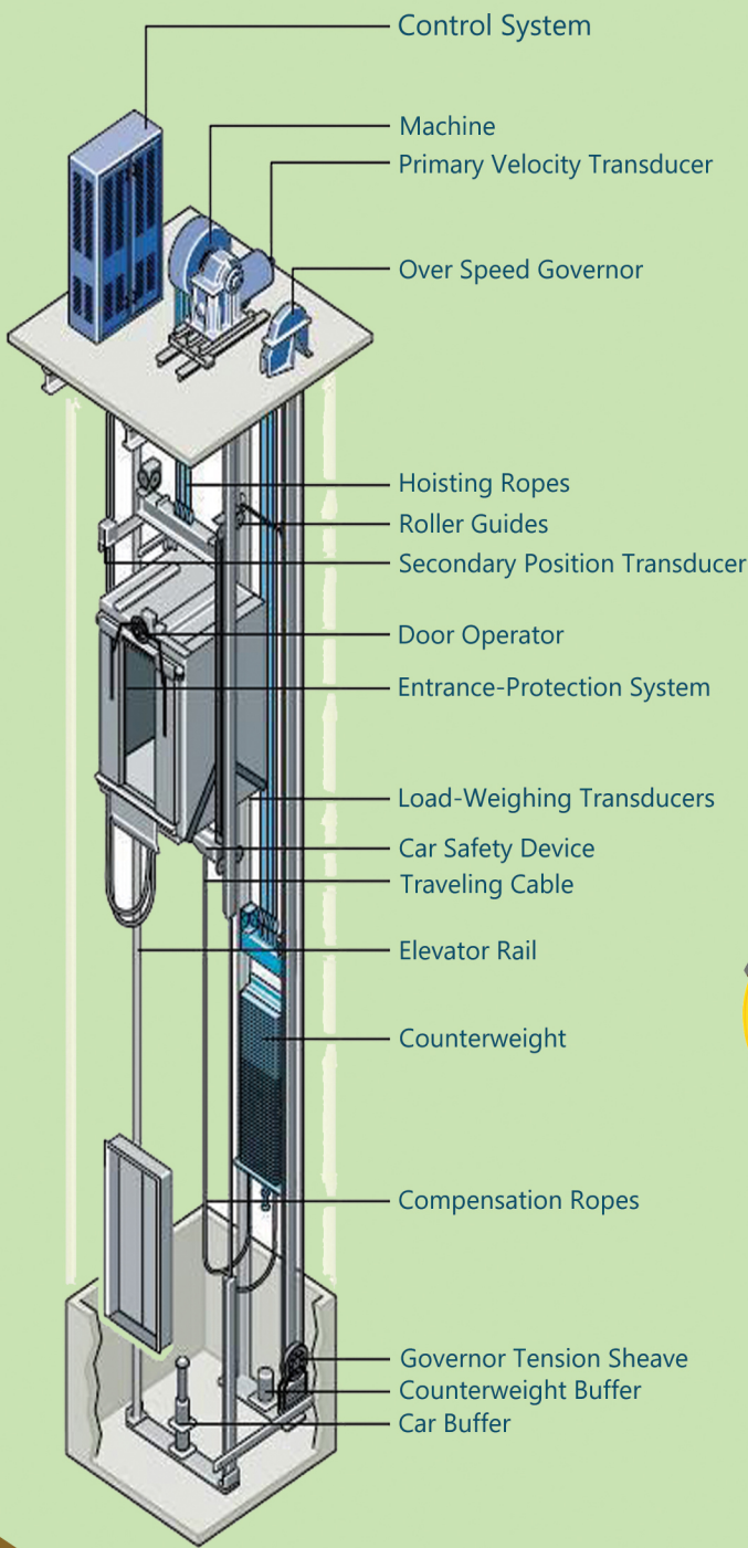
Gear Less Machine
