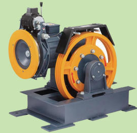
Traction Machines
